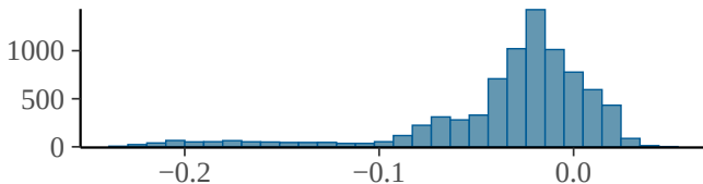
bs_t2EastingNorthingdate_index_5
