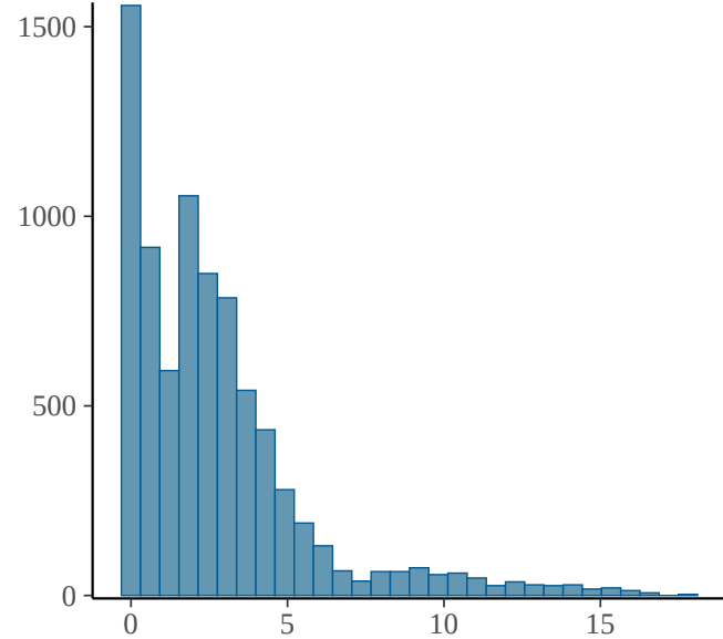
sds_t2EastingNorthingdate_index_2
