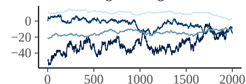
bs_t2EastingNorthingdate_index_4
