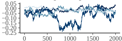
bs_t2EastingNorthingdate_index_5
