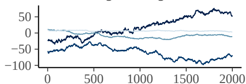
bs_t2EastingNorthingdate_index_2
