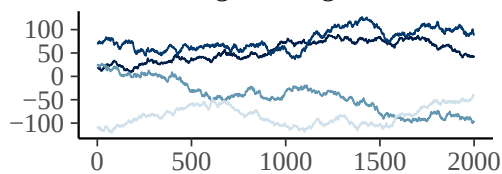
bs_t2EastingNorthingdate_index_1
