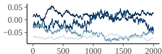
b_scale_imd_score
