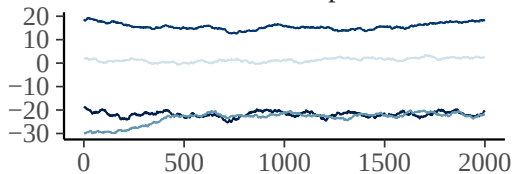
b_Intercept
