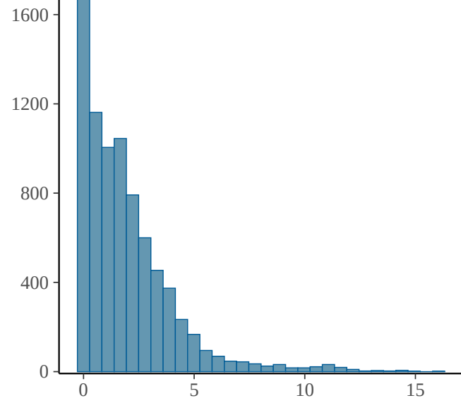
sds_t2EastingNorthingdate_index_3
