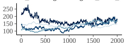
sds_t2EastingNorthingdate_index_1
