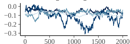
bs_t2EastingNorthingdate_index_3
