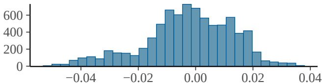
b_scale_mobility
