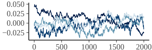
b_scale_temp_rolling_7day
