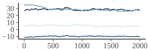
b_lockdown_lifting
