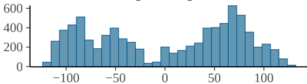
bs_t2EastingNorthingdate_index_1
