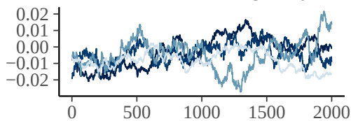
b_scale_rain_rolling_7day
