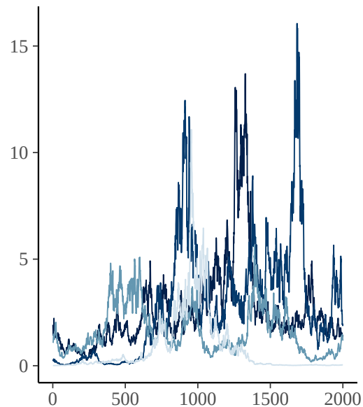
sds_t2EastingNorthingdate_index_3
