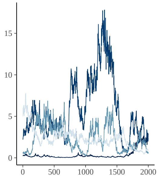
sds_t2EastingNorthingdate_index_2
