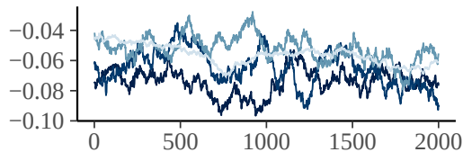
b_scale_school_density
