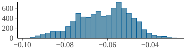
b_scale_school_density
