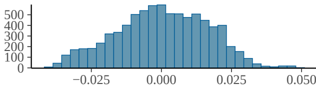
b_scale_temp_rolling_7day
