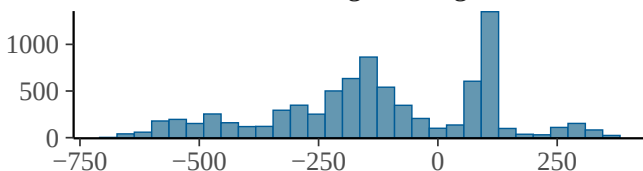
bs_sEastingNorthing_1
