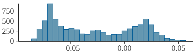
b_scale_imd_score
