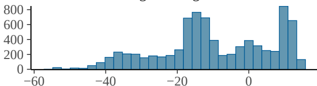
bs_t2EastingNorthingdate_index_4
