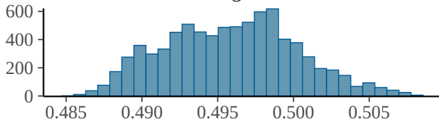
sigma
