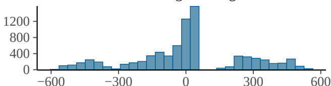
bs_sEastingNorthing_2
