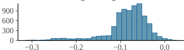
bs_t2EastingNorthingdate_index_3
