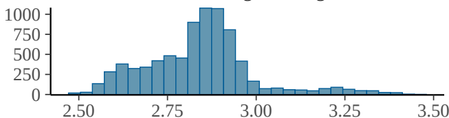
sds_sEastingNorthing_1
