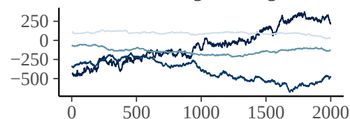
bs_sEastingNorthing_1
