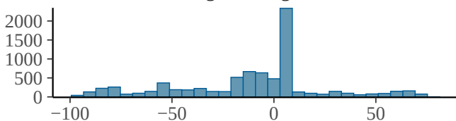
bs_t2EastingNorthingdate_index_2
