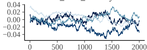
b_scale_mobility
