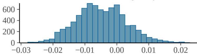
b_scale_rain_rolling_7day
