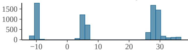
b_lockdown_lifting
