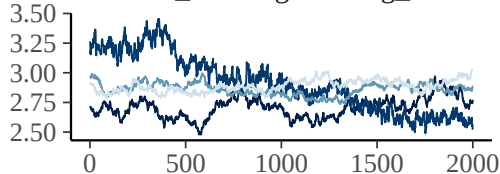
sds_sEastingNorthing_1
