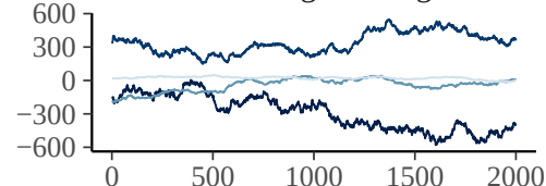
bs_sEastingNorthing_2
