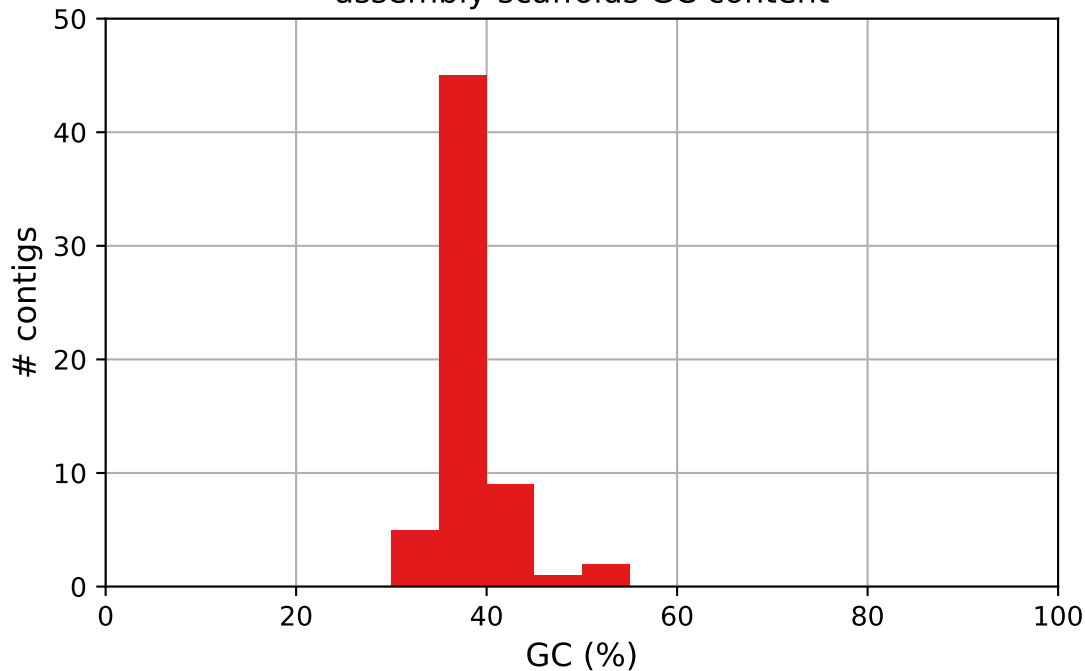
assembly-scaffolds GC content
