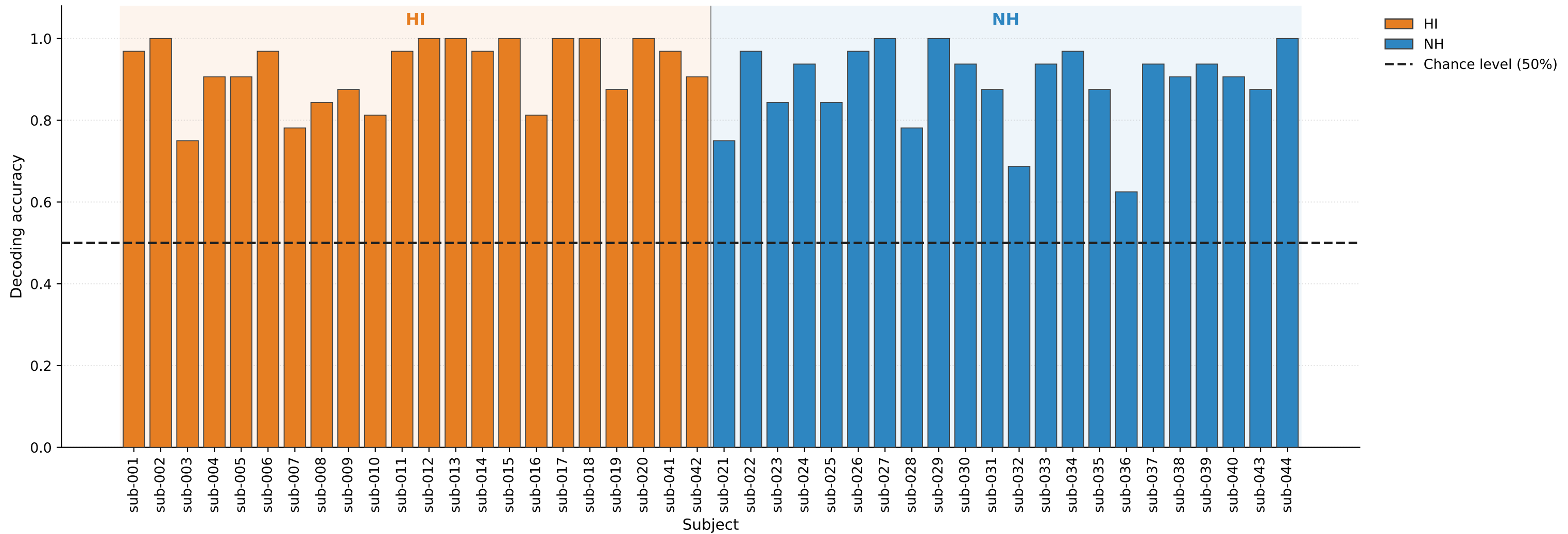
Envelope baseline AAD: subject-wise decoding accuracy (scalp EEG only)
