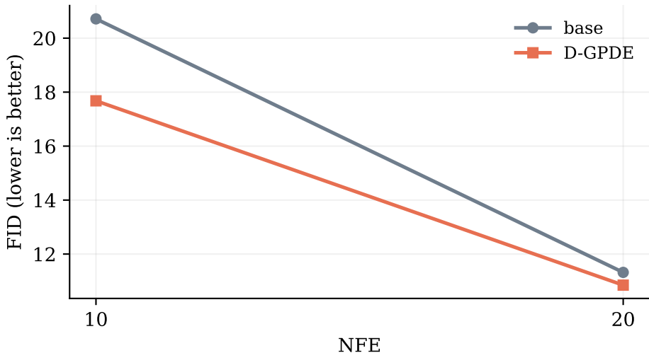
PNDM/CIFAR-10 Euler, 50k samples, seed 0
