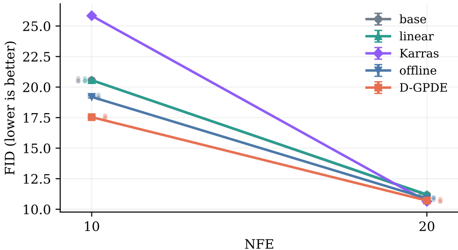
PNDM/CIFAR-10 Euler, 50k samples, seeds 0/1/2
