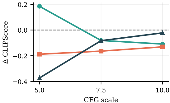
CLIPScore
