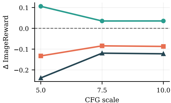
ImageReward
