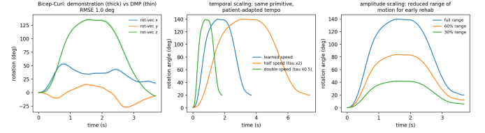
Fig. 4. Left: DMP reconstruction over the demonstration. Middle, right: temporal and amplitude scaling of one learned primitive.
