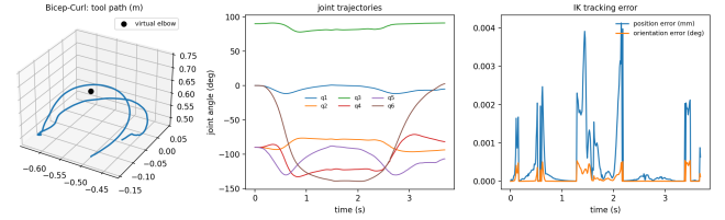
Fig. 6. Retargeting one learned bicep-curl repetition to the UR5e. Left: the commanded tool path traced about the virtual elbow anchor. Middle: the six resulting joint trajectories. Right: inverse-kinematic tracking error, which stays below 0.005 mm and 0.0006^\circ for this exercise.
