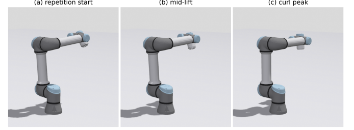
Fig. 5. The UR5e executing a learned Bicep-Curl primitive in Gazebo (camera frames from the simulated therapy set). Under the single-pivot retargeting, the exercise is carried by the tool’s orientation: the wrist sweeps the demonstrated hand arc from the hanging start pose (a) through mid-lift (b) to the curl peak (c).
