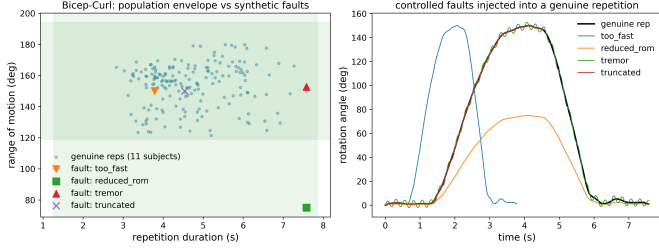
Fig. 7. Left: population envelope (shaded) for one exercise with fault positions of one repetition. Right: the injected fault types.
