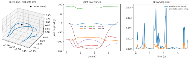
Fig. 6. Retargeting one learned bicep-curl repetition to the UR5e. Left: the commanded tool path traced about the virtual elbow anchor. Middle: the six resulting joint trajectories. Right: inverse-kinematic tracking error, which stays below 0.005 mm and 0.0006° for this exercise.
