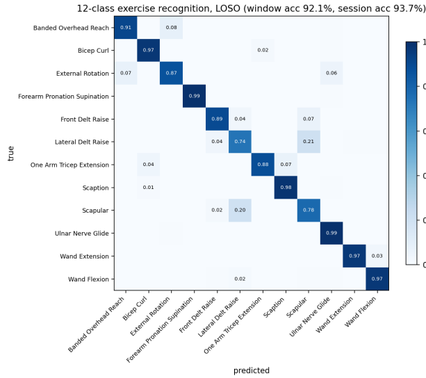
Fig. 2. 12-class LOSO confusion matrix (window level, all folds).
