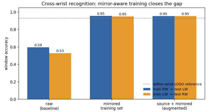
Fig. 3. Cross-wrist recognition with raw, mirrored, and augmented training. The dashed line is the within-wrist LOSO reference.
