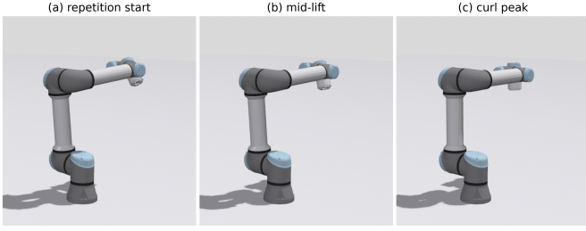
Fig. 6. The UR5e executing a learned Bicep-Curl primitive in Gazebo (camera frames from the simulated therapy set). Under the single-pivot retargeting, the exercise is carried by the tool’s orientation: the wrist sweeps the demonstrated hand arc from the hanging start pose (a) through mid-lift (b) to the curl peak (c).
