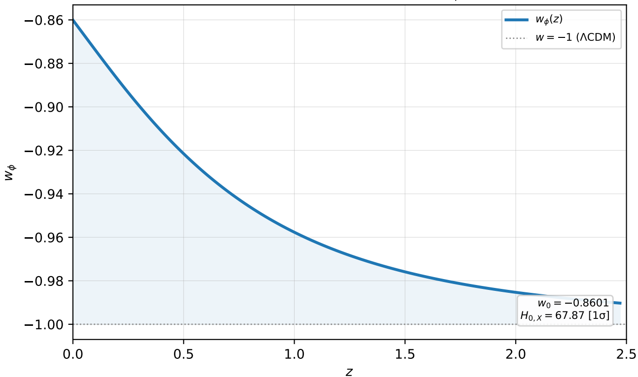
WLI_2 — equation of state w_\phi(z)
