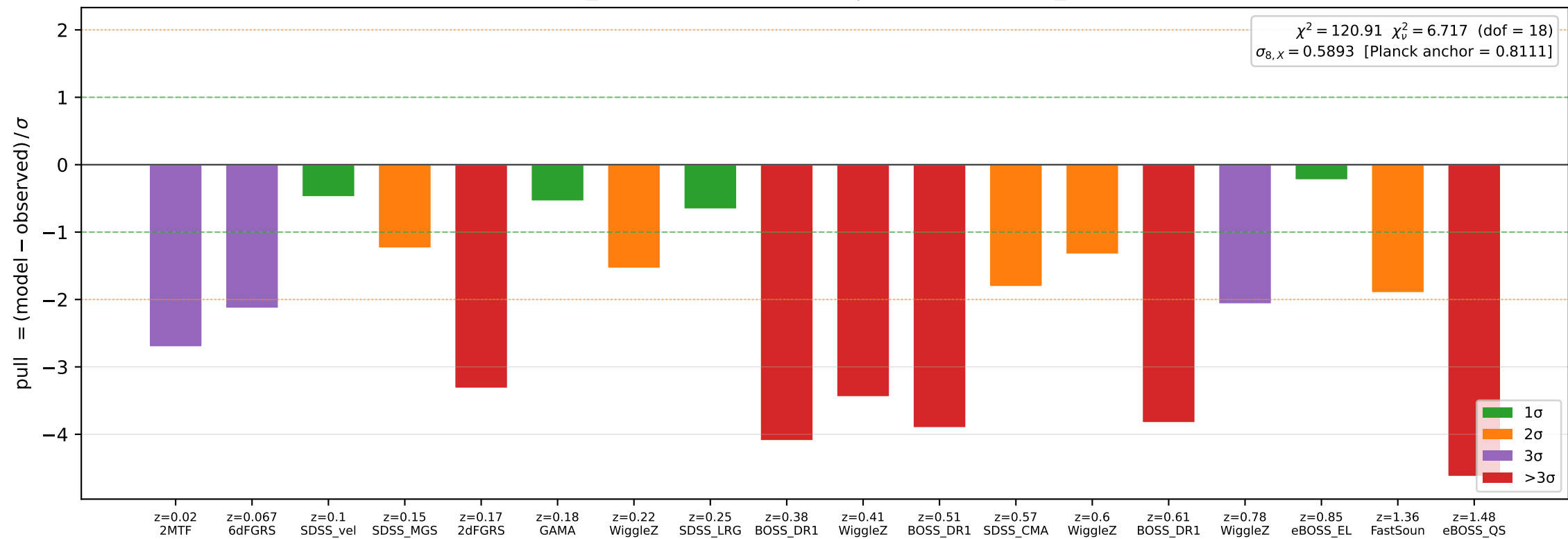
WLI_3 — RSD f\sigma_8 pulls ( H_{0,x} = 68.20 , LOOSE_2S)
