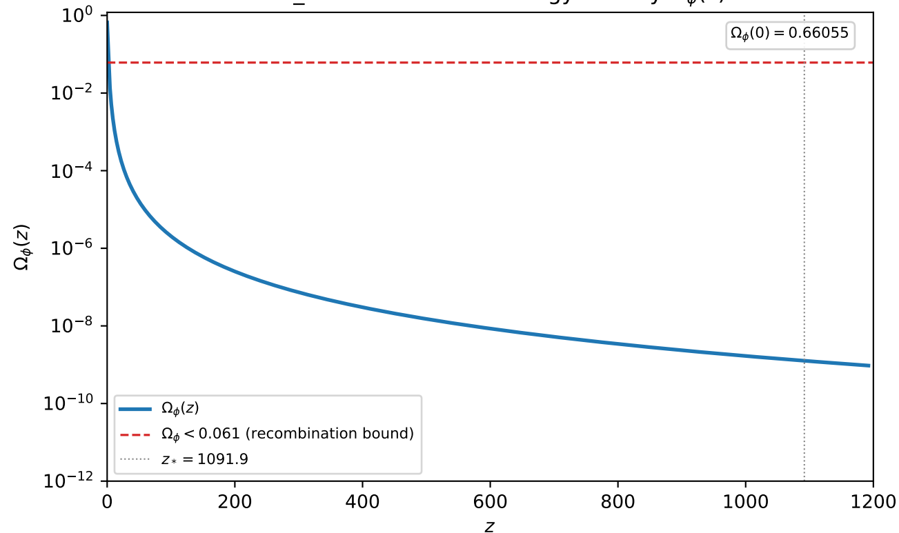
WLI_1 — scalar-field energy density \Omega_\phi(z)
