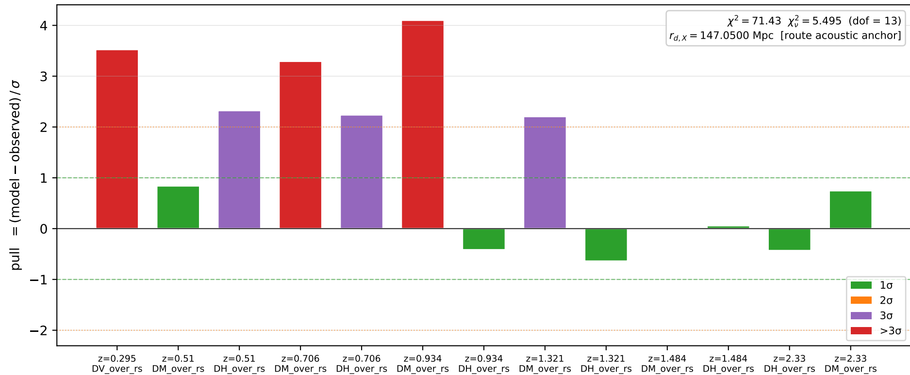
WLI_1 — DESI DR2 BAO pulls ( H_{0,x} = 65.15 , LOOSE_3S)
