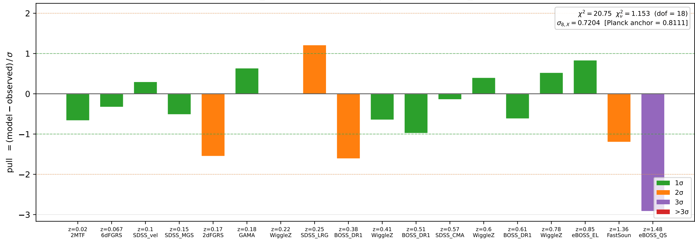
WLI_1 — RSD f\sigma_8 pulls ( H_{0,X} = 65.15 , LOOSE_3S)
