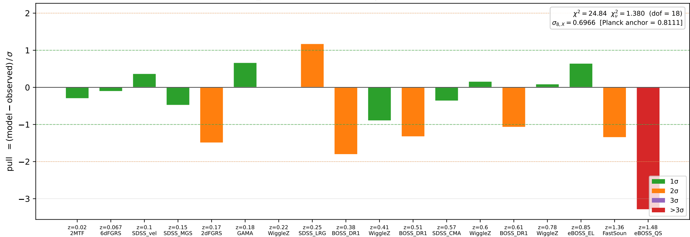
WLI_3 — RSD f\sigma_8 pulls ( H_{0,X} = 60.39 , EXCLUDED)
