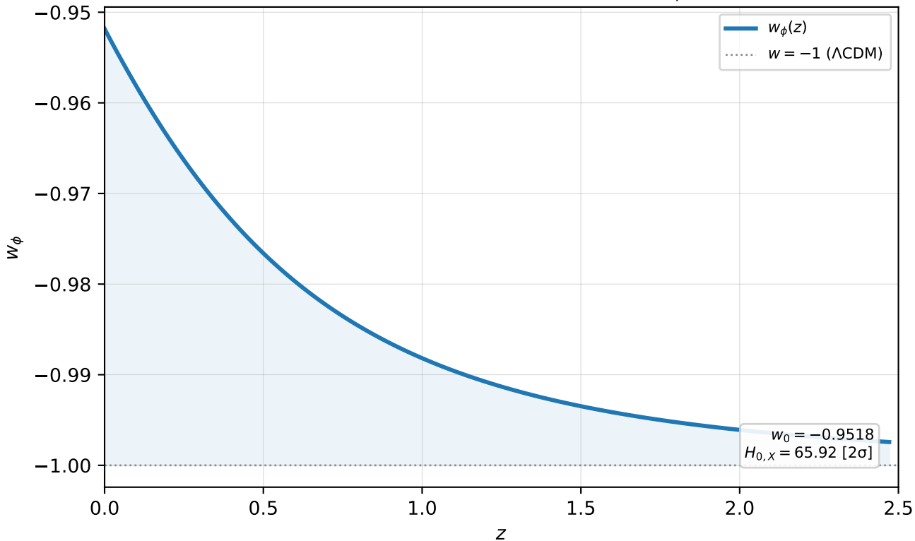
WQI_F680 — equation of state w_\phi(z)
