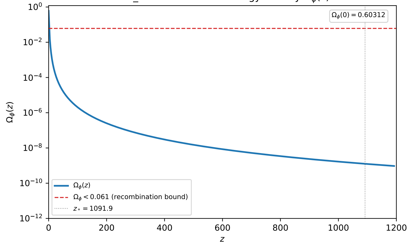
WLI_6 — scalar-field energy density \Omega_\phi(z)
