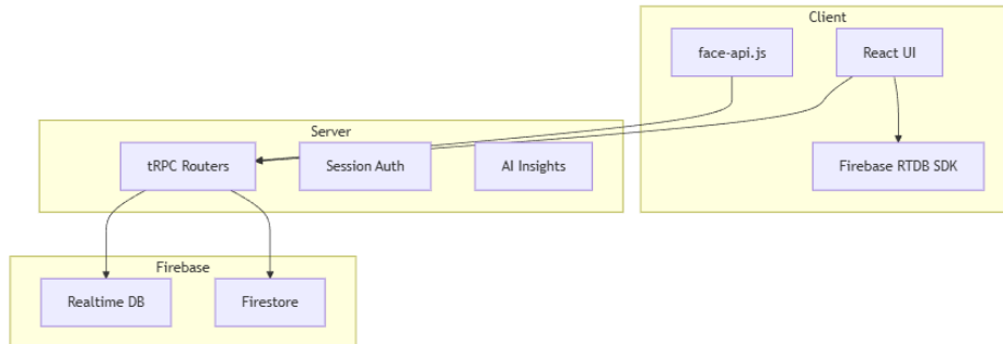
Figure 3.3: System-wide software architecture and module boundaries.
