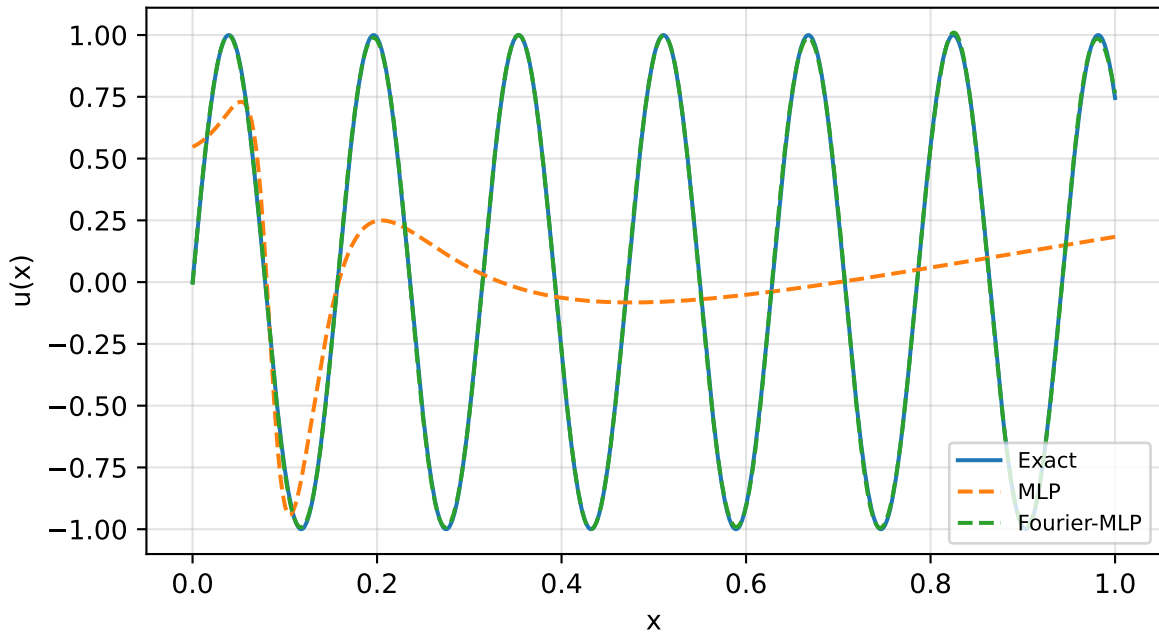
Function fitting: \sin(40 x)
