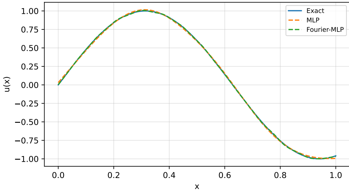
Function fitting: \sin(5x)
