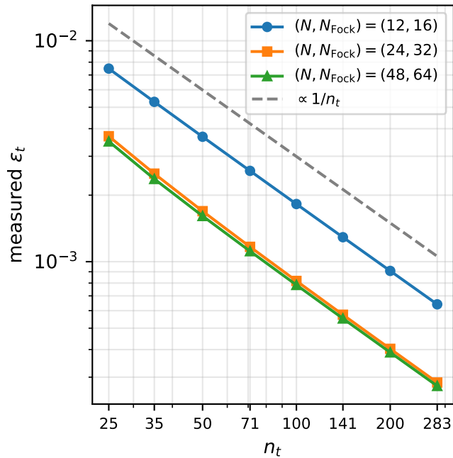
(b) product-formula error at T = 1
