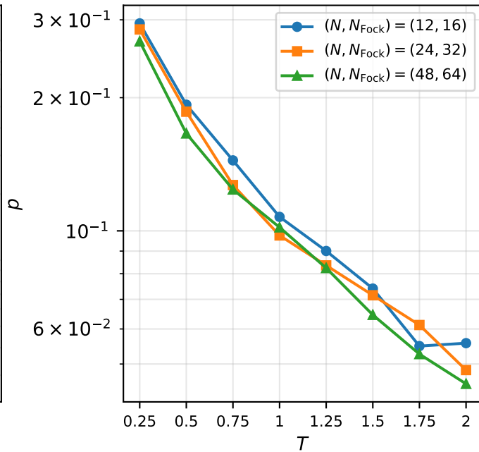
(c) postselection probability vs. time
