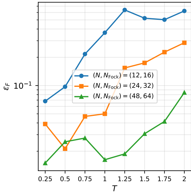
(a) map error vs. evolution time
