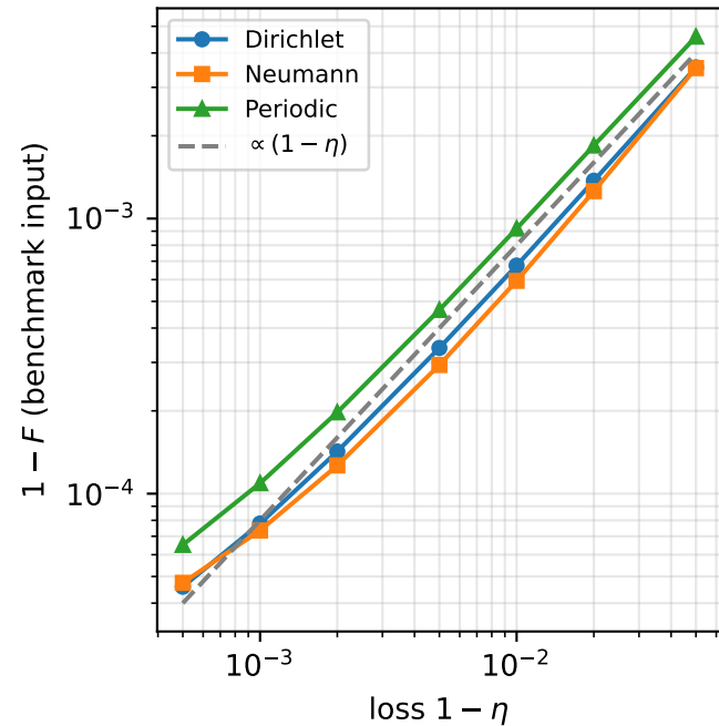
(a) conditional infidelity vs. loss
