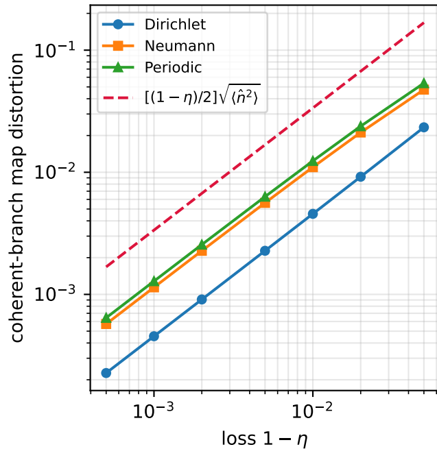
(b) coherent-branch map distortion
