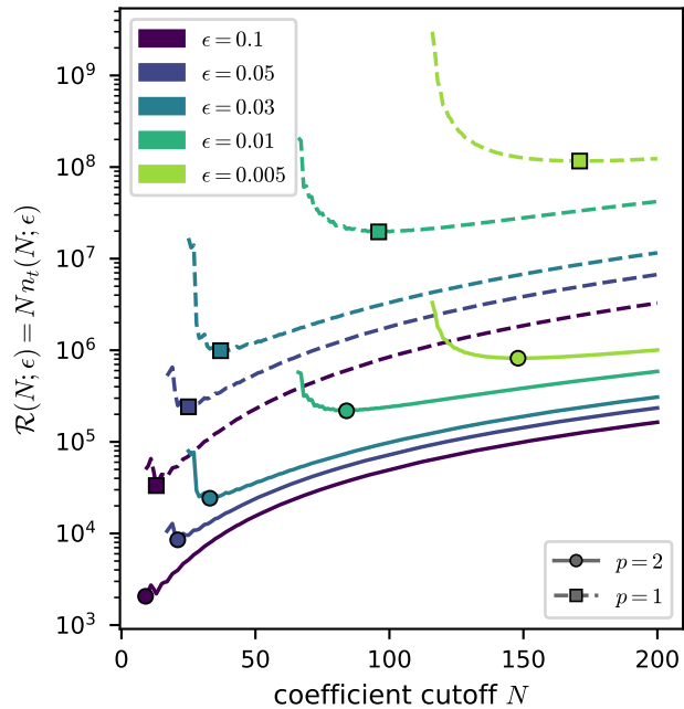
(b) joint proxy, N_{\text{Fock}} = \lceil 2N \rceil
