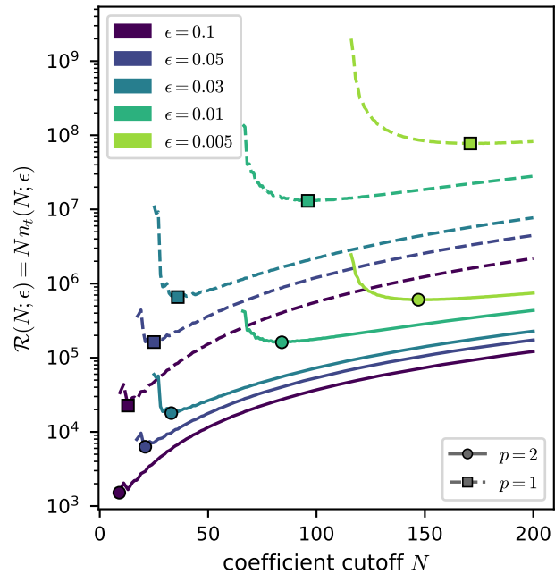
(c) joint proxy, N_{\text{Fock}} = \lceil 4/3 N \rceil
