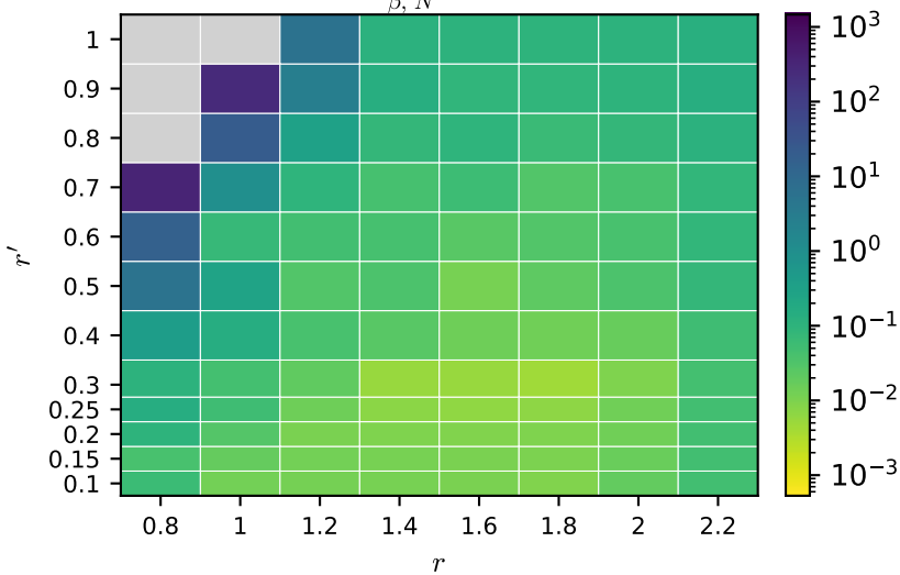
Dirichlet: \min_{\beta, N} \varepsilon_F over (r, r')
