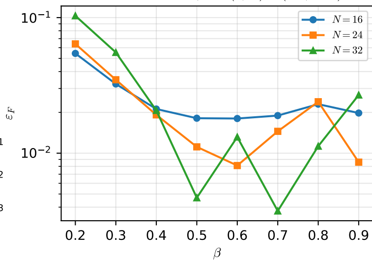
Periodic: \varepsilon_F vs \beta at (r, r') = (1.6, 0.25)
