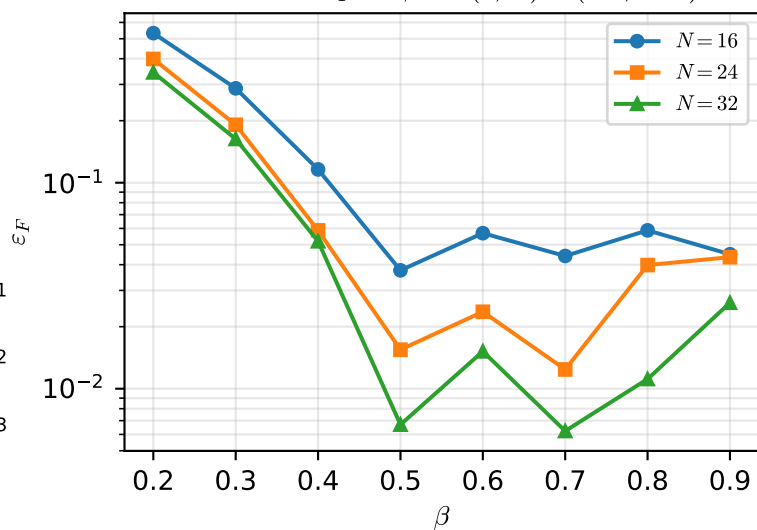
Dirichlet: \varepsilon_F vs \beta at (r, r') = (1.6, 0.25)
