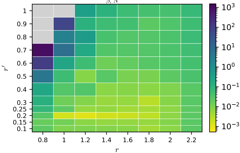
Neumann: \min_{\beta, N} \varepsilon_F over (r, r')
