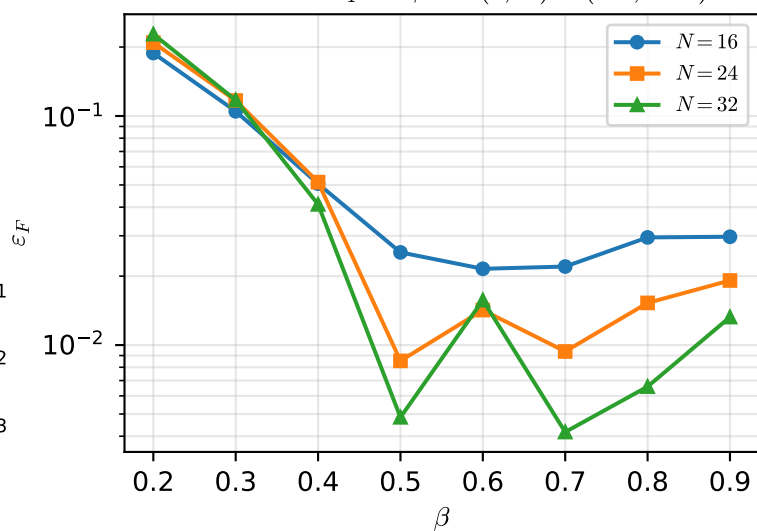
Neumann: \varepsilon_F vs \beta at (r, r') = (1.6, 0.25)
