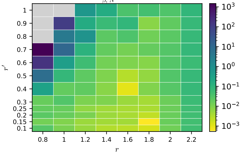
Periodic: \min_{\beta, N} \varepsilon_F over (r, r')
