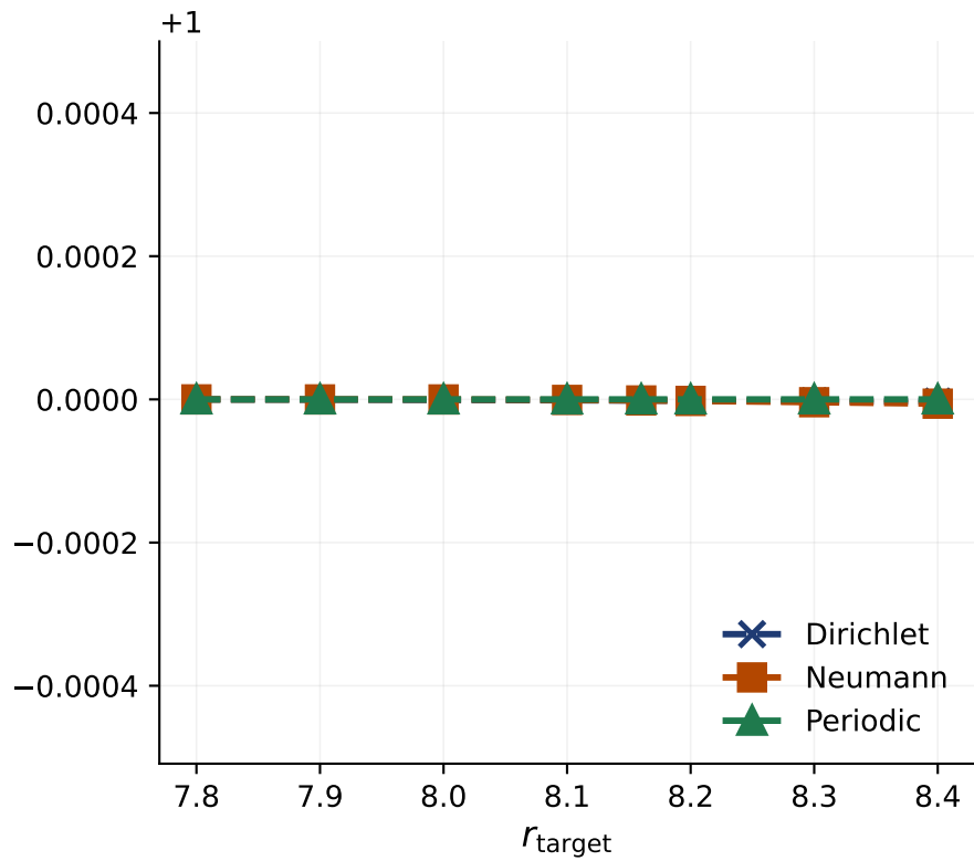
Truncated-model fidelity
