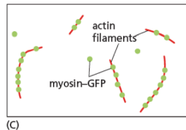
Figure 9–32 TIRF microscopy allows the detection of single fluorescent molecules. (A) TIRF microscopy uses excitatory laser light to illuminate the cover-slip surface at the critical angle at which all the light is reflected by the glass–water interface. Some electromagnetic energy extends a short distance across the interface as an evanescent wave that excites just those molecules that are attached to the cover slip or are very close to its surface. (B) TIRF microscopy is used here to image individual myosin–GFP molecules (green dots) attached to nonfluorescent actin filaments (C), which are invisible but stuck to the surface of the cover slip. (Courtesy of Dmitry Cherny and Clive R. Bagshaw.)
