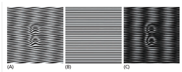
Figure 9-34 Structured illumination
