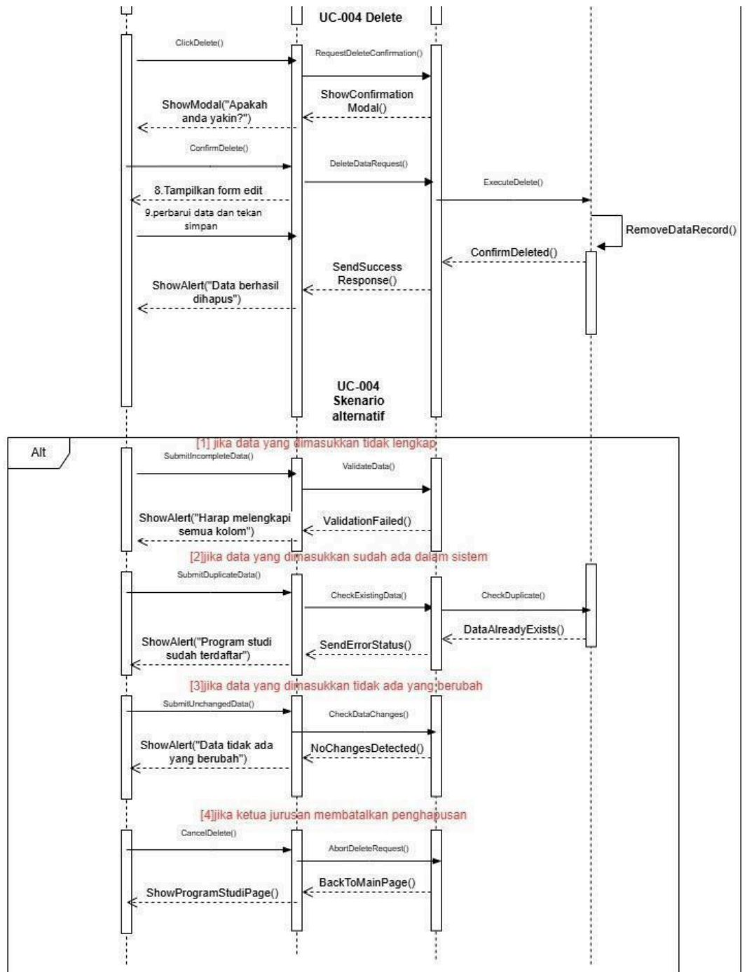
gambar 3.5 sequence diagram mengelola program studi
