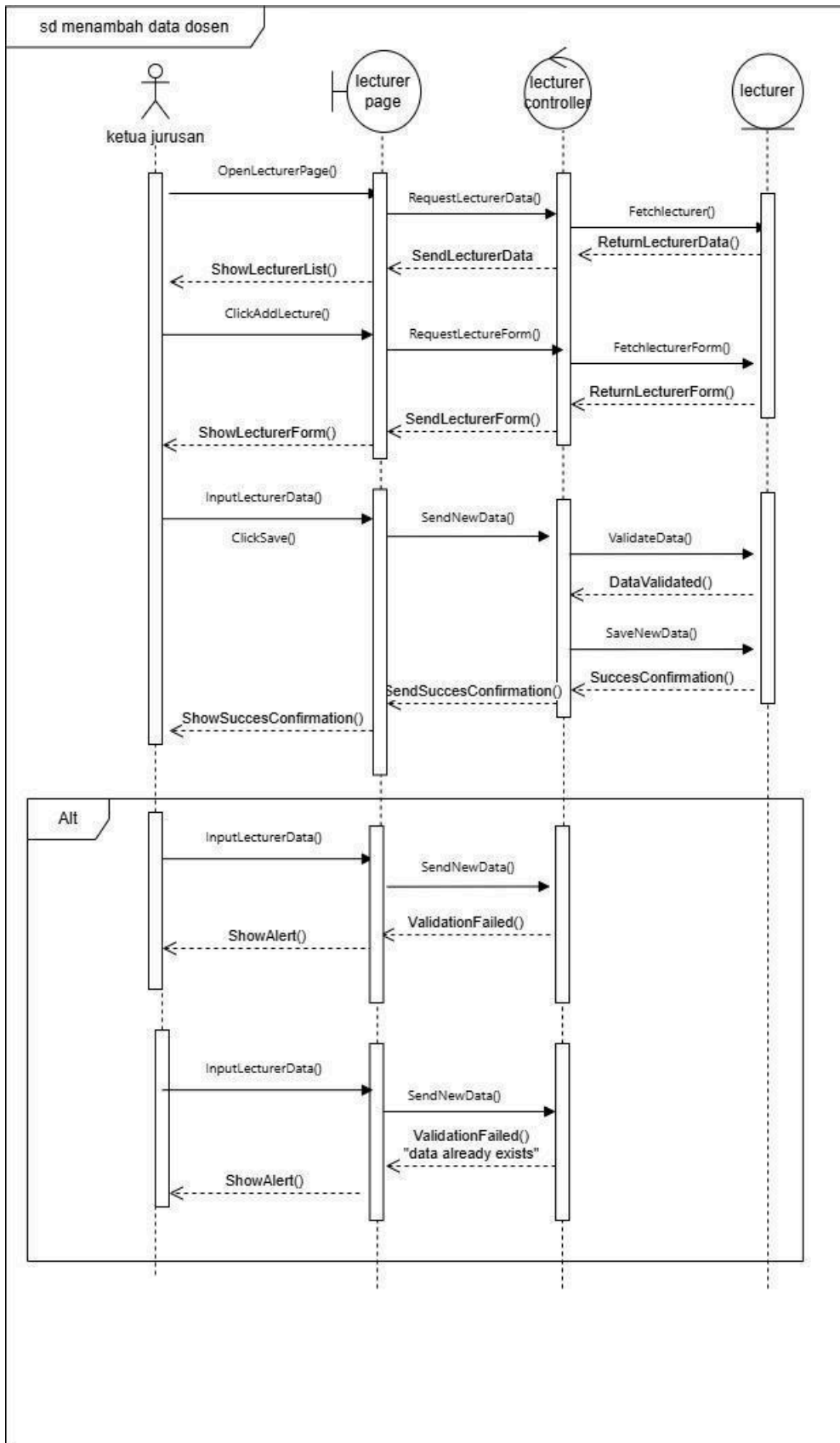
gambar 3.16 sequence diagram mengelola data dosen
