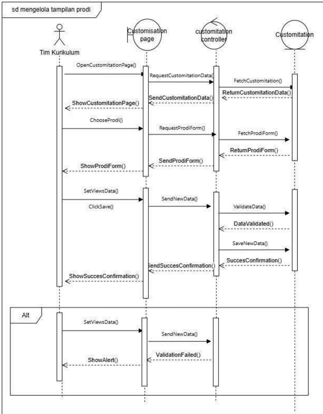
gambar 3.17 sequence diagram mengelola tampilan program studi
