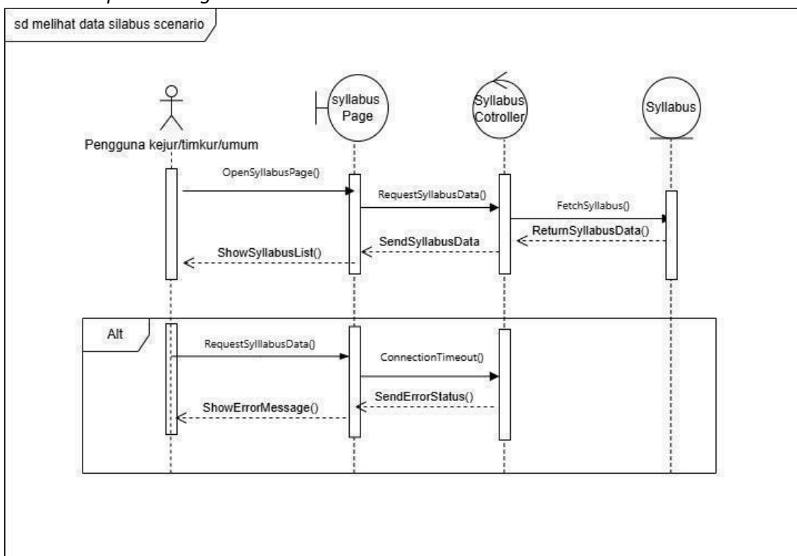
gambar 3.15 sequence diagram melihat data silabus
