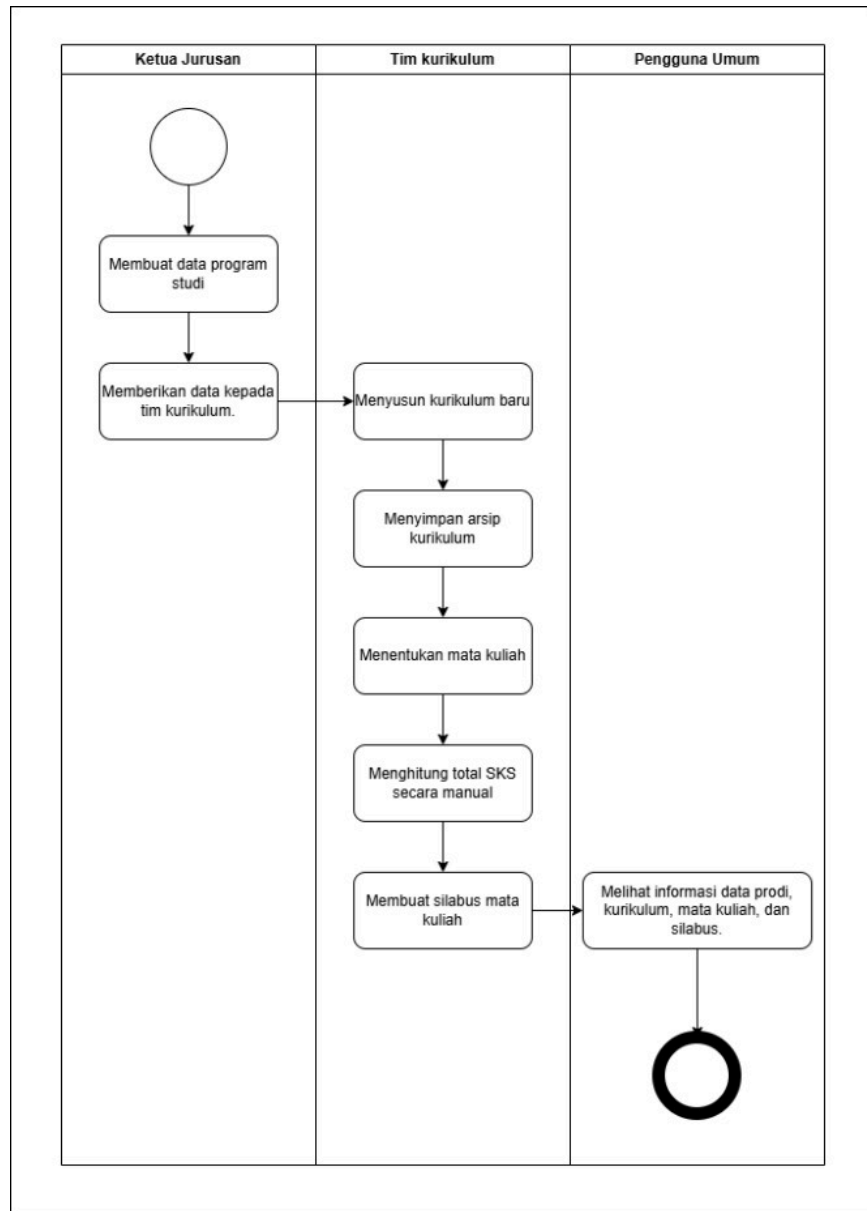
gambar 2.3 diagram activity current
