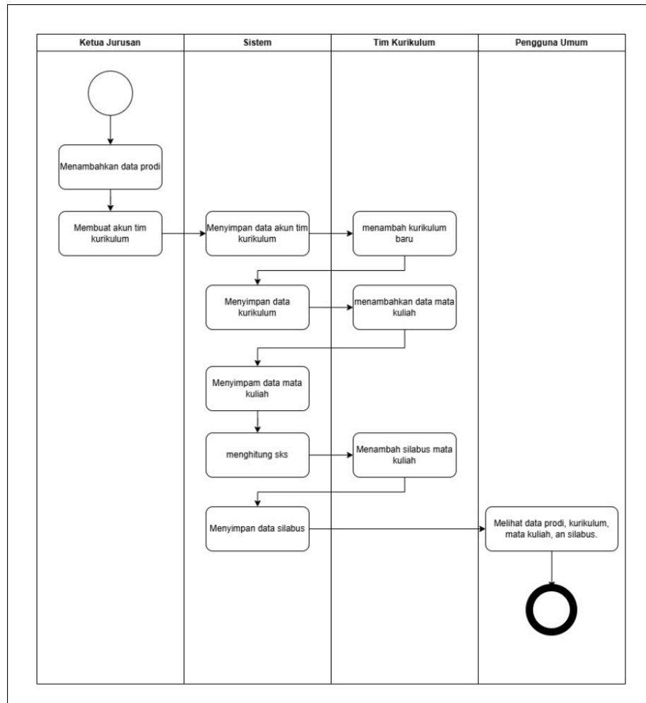
gambar 2.4 diagram activity to be
