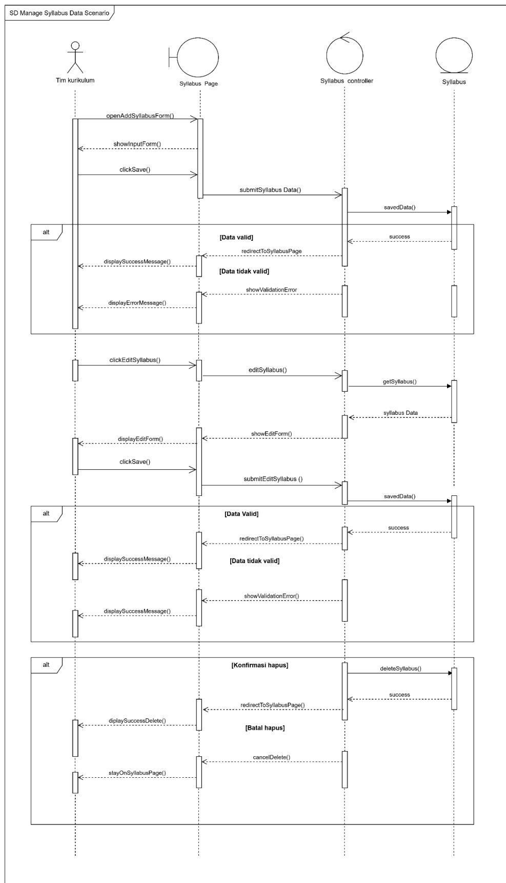
gambar 3.10 sequence diagram mengelola data silabus
