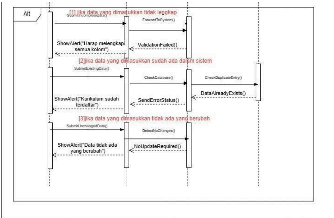
gambar 3.7 sequence diagram mengelola kurikulum
