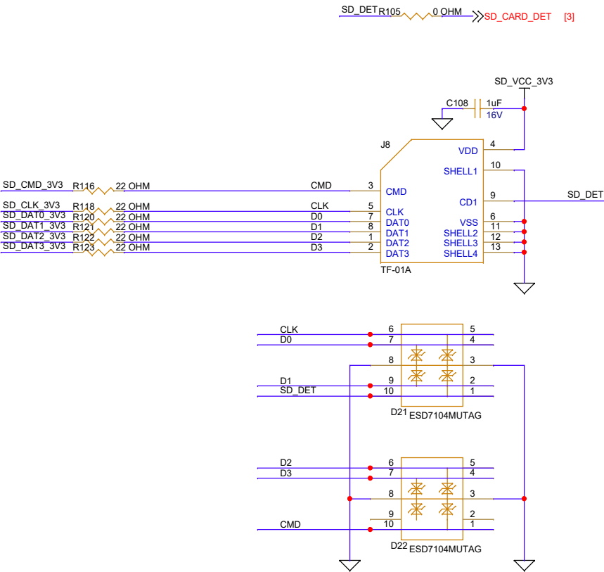
microSD Card Interface
