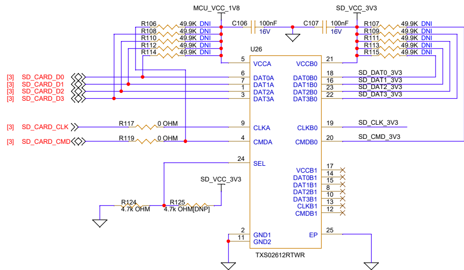
Level Translator for microSD Card
