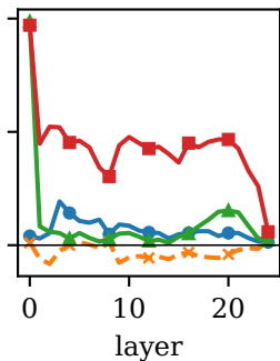
w2v-BERT 2.0
