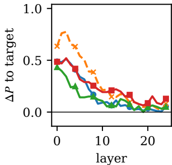
WavLM
