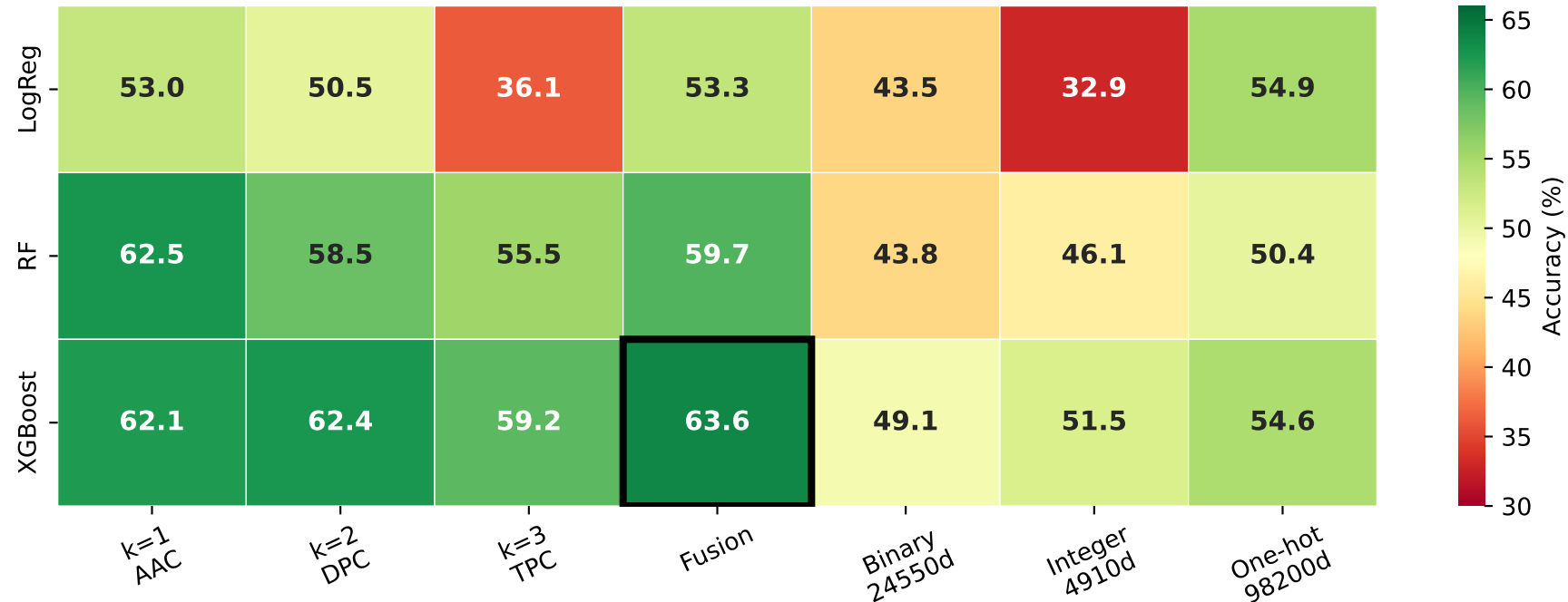
Model x Encoding Accuracy (% , mean of 3 seeds)
