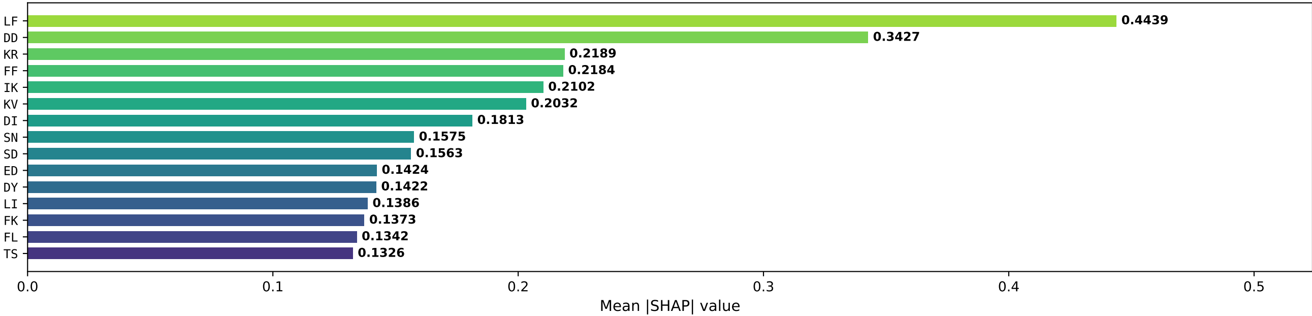
A Overall Top-15 Dipeptide Features (SHAP Importance)
