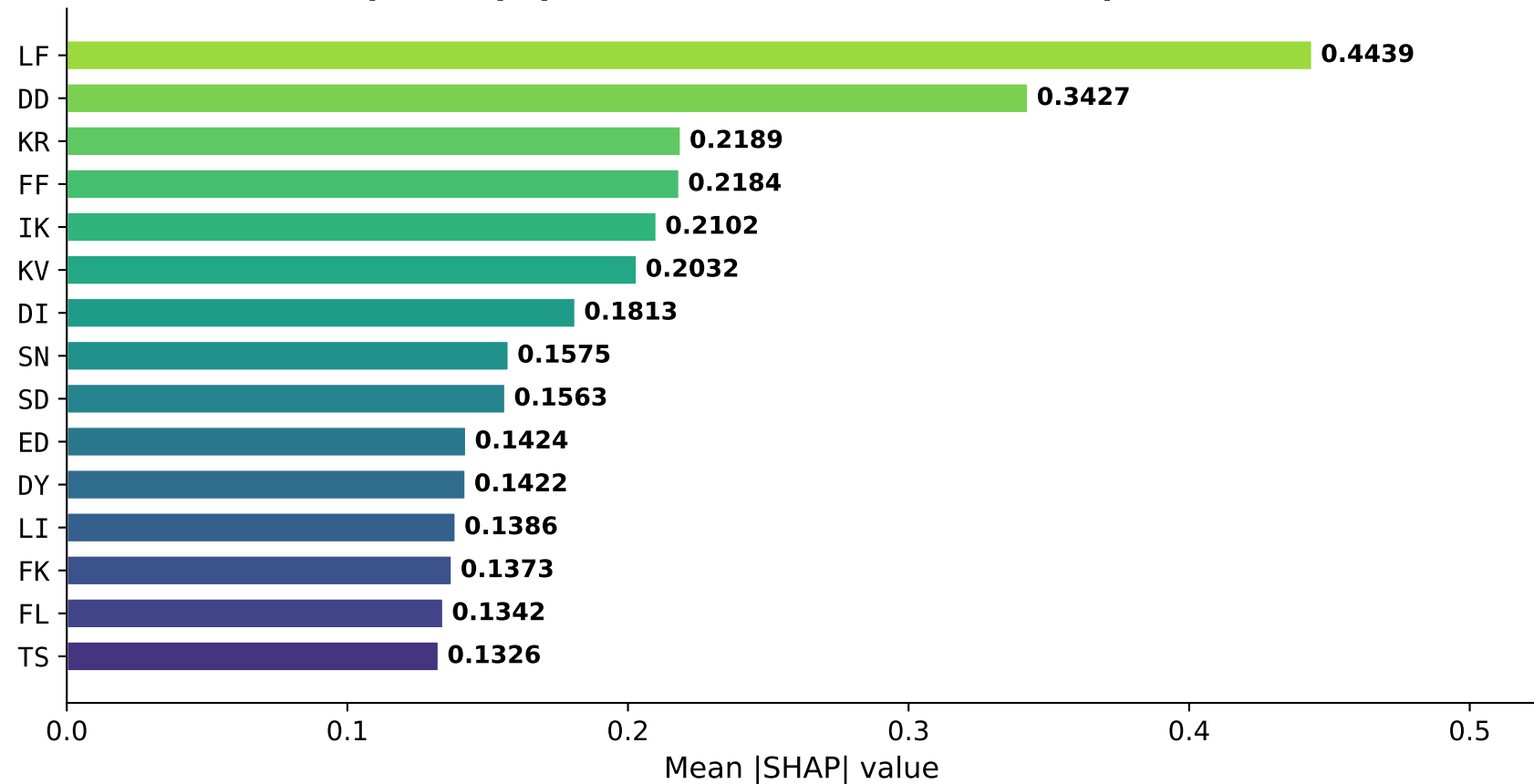
Top-15 Dipeptide Features (SHAP Global Importance)
