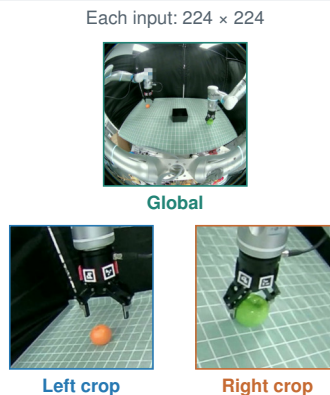
Figure 1: Fisheye-VLA uses one fixed camera (boxed) to supply a global view and two interaction-centered crops, each 224 \times 224 . White outlines mark the 90^\circ front-camera field of view. Rendering local detail from the wider fisheye image supports manipulation without wrist cameras.
