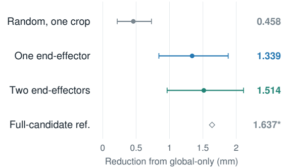
Figure 3: Evaluation geometry and crop-placement gains. (a) Top view of the tabletop: R1–R3 denote increasingly large placement extents, with the camera on the robot side. (b) Round 2 endpoint-error reductions relative to the global-only input, with 95% episode-clustered intervals; the diamond is the derived full-candidate reference. EE-centered views account for most of the estimated reduction.
