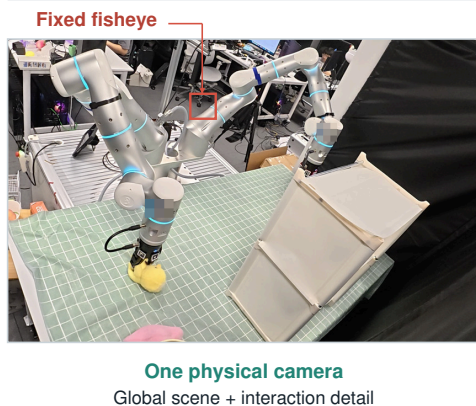
Figure 1: Fisheye-VLA uses one fixed camera (boxed) to supply a global view and two interaction-centered crops, each 224 \times 224 . White outlines mark the 90^\circ front-camera field of view. Rendering local detail from the wider fisheye image supports manipulation without wrist cameras.
