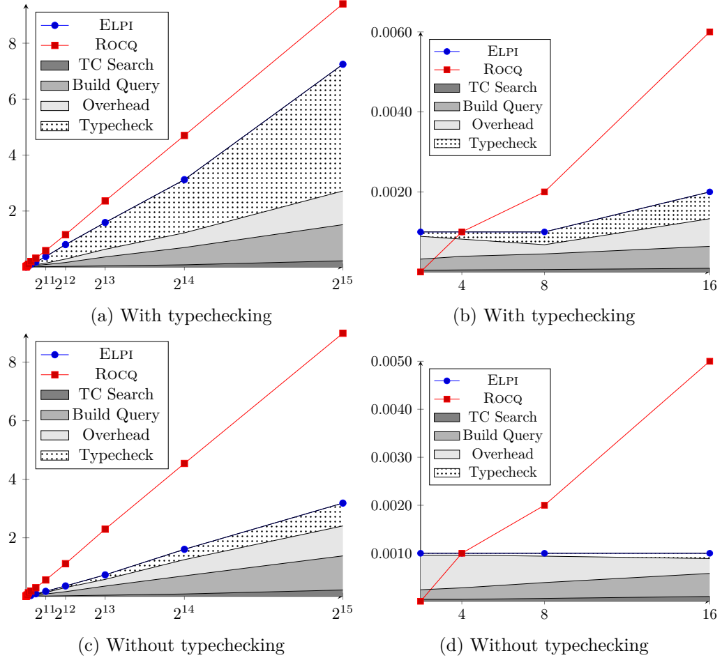
Figure 3.7: Benchmarks of the ELPI solver. The x-axis of each plot represents the problem size, expressed as the number of nodes. The y-axis represents the resolution time, expressed in seconds.
