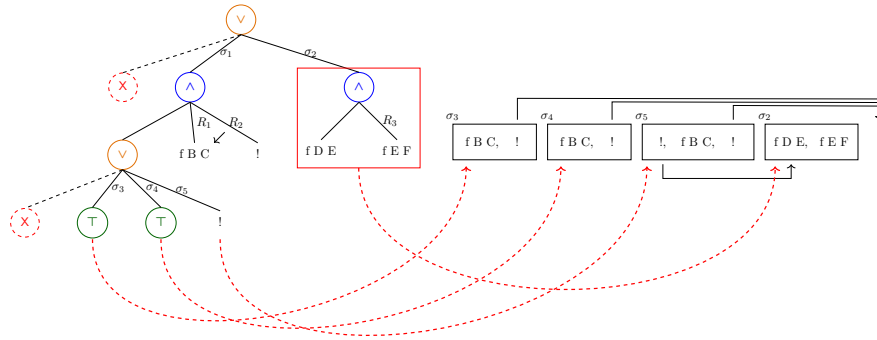
Figure 6.8: Example of \mathsf{t2l} execution
