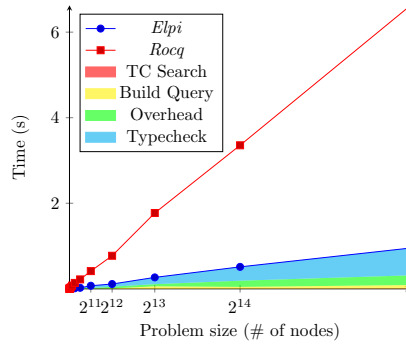
(b) Benchmark with memory sharing
