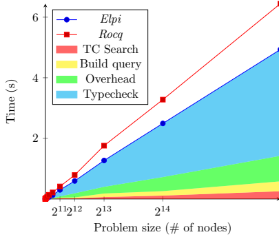
(a) Benchmark with typechecking
