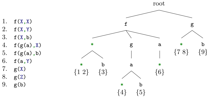
Figure 5.1: Example of a discrimination tree, from [41]
