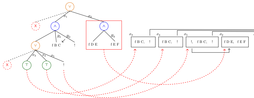
Figure 6.8: Example of \tau_{21} execution
