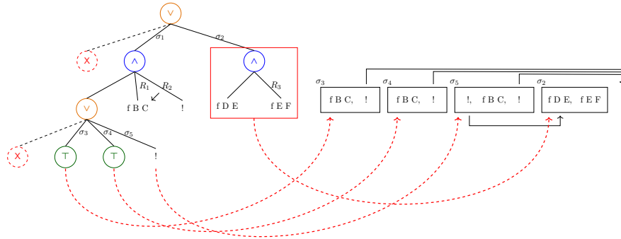
Figure 6.10: Example of t2l execution
