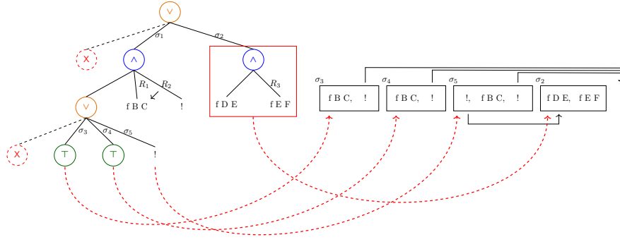
Figure 6.9: Example of tree_to_stack execution
