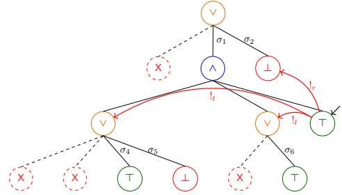
(d.2) prune on Figure 5d.1
