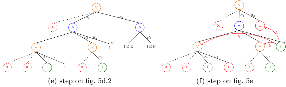
Fig. 5: Execution in the tree semantics. The substitutions \sigma_1 \dots \sigma_6 are from section 2.1. R_1 , R_2 , and R_3 are reset points and correspond respectively to the lists of atoms [f \ Y \ Z, !] , [!] , and [f \ Y \ Z] .
