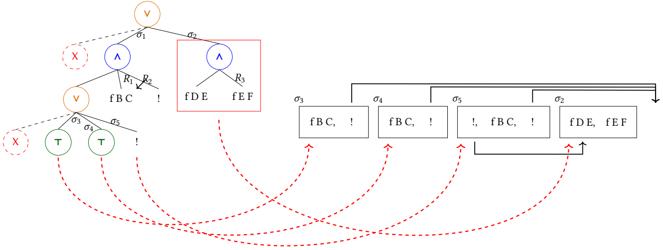
Figure 8. Example of t2s execution
