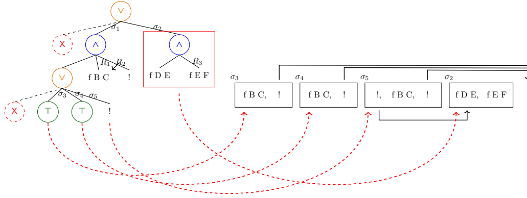
Figure 8. Example of t2s execution
