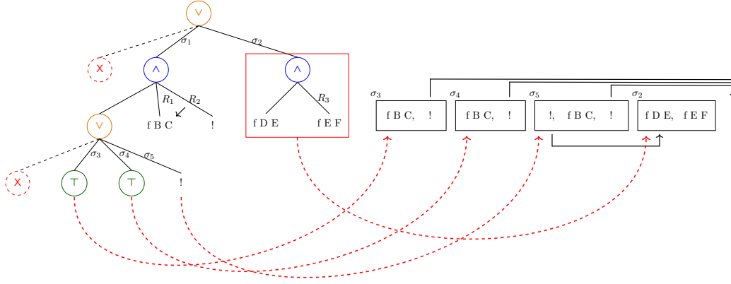
Figure 10. Example of tree_to_stack execution
