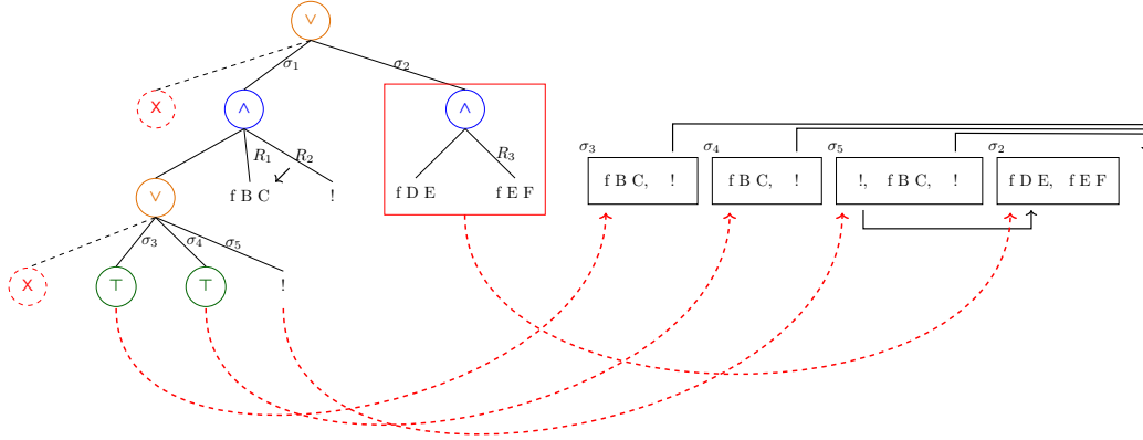
Figure 8. Example of tree_to_stack execution
