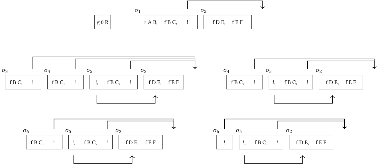
Figure 3. Example of execution
