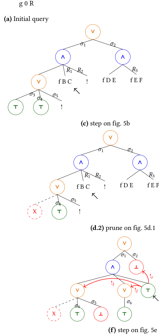
Figure 5. Execution in the tree semantics. The substitutions \sigma_1 \dots \sigma_6 are from section 2.1. R_1, R_2 , and R_3 are reset points and correspond respectively to the lists of atoms [f \ B \ C, !] , [!] , and [f \ E \ F] .
