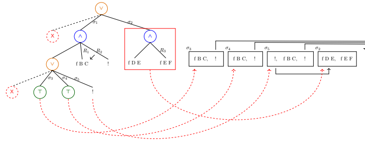
Fig. 9: Example of t2l execution
